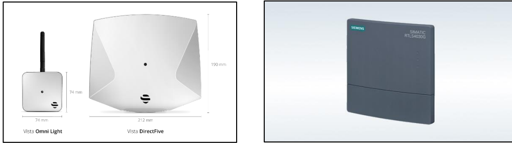
20. ábra - RTLS Anchor-ok [29], [30]
